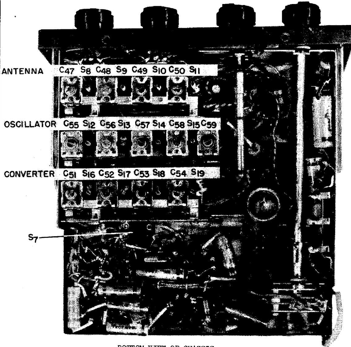
BOTTOM VIEW OF CHASSIS
