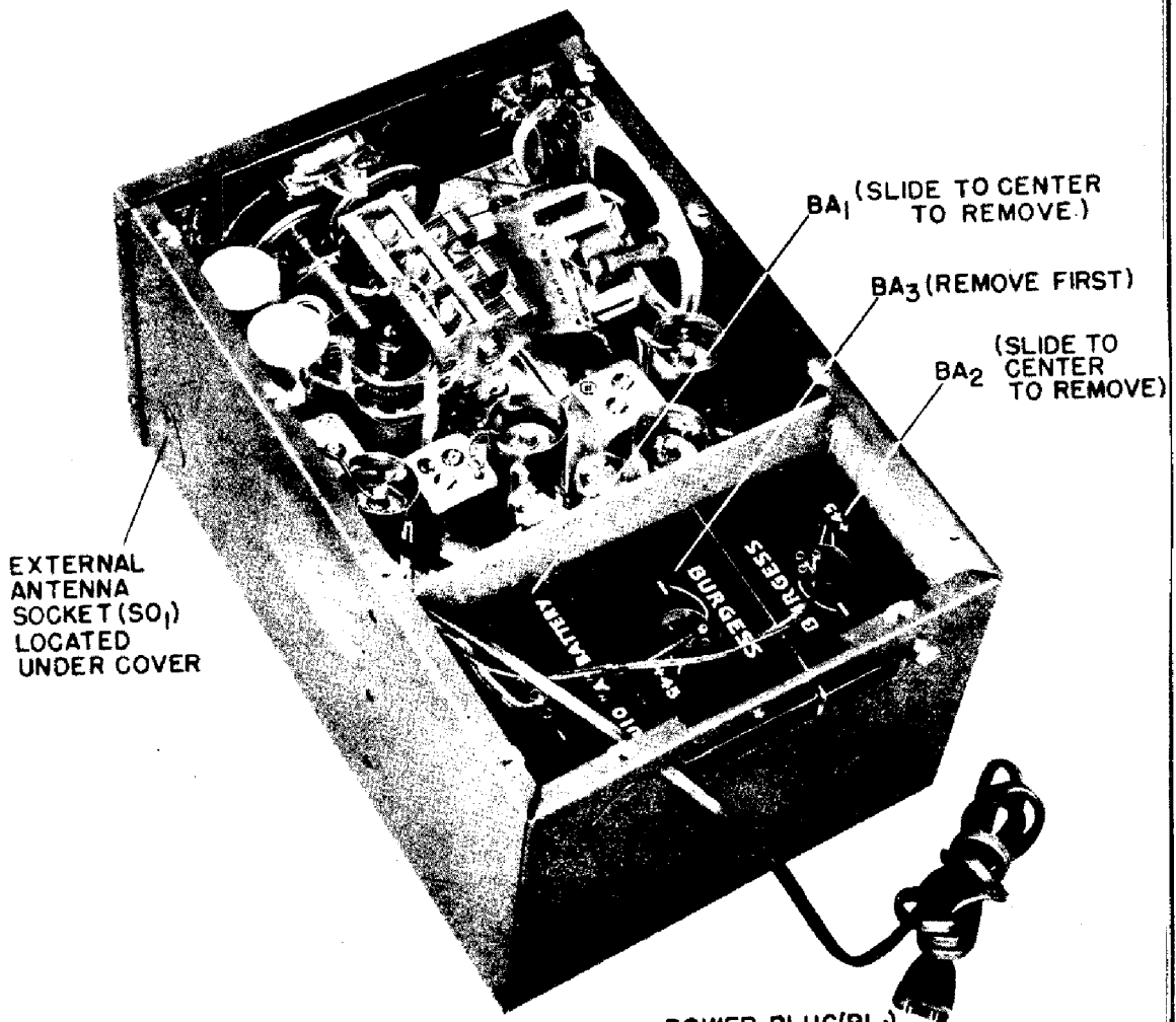
MODEL S-39 RECEIVER, REAR VIEW, COVER REMOVED, SHOWING POWER CORD COMPARTMENT AND BATTERY COMPARTMENT.
